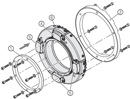
Mounting option 1
