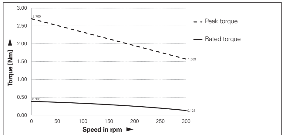
Characteristic curve of torque at DC 48 V
