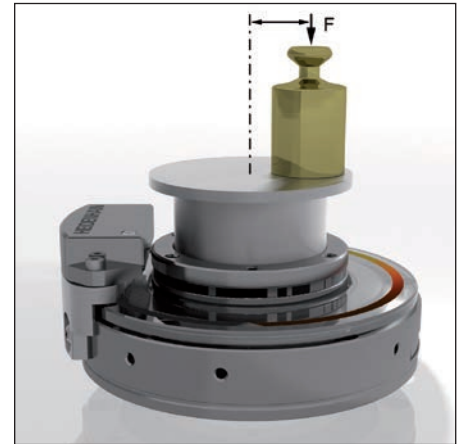
Figure 2: Off-center load
