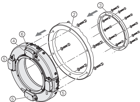
Mounting option 2
