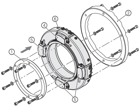
Mounting option 1
