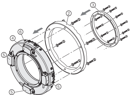
Mounting option 2
